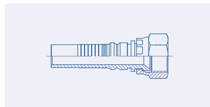
Interlock Female JIC 37° Swivel (DKJ)
